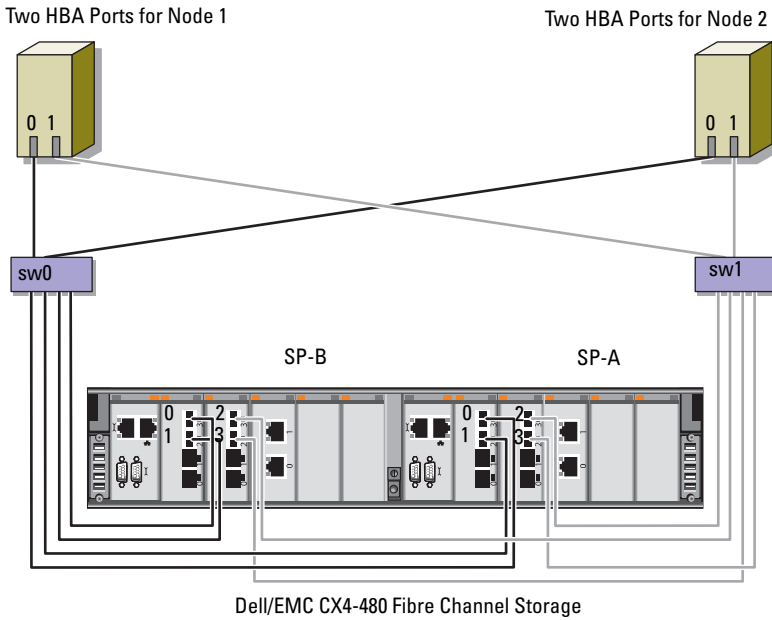
Figure 3-3. Cabling in a SAN-Attached Fibre Channel Cluster
