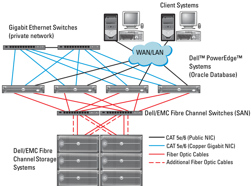
Figure 3-1. Hardware Connections for a Fibre Channel Cluster
