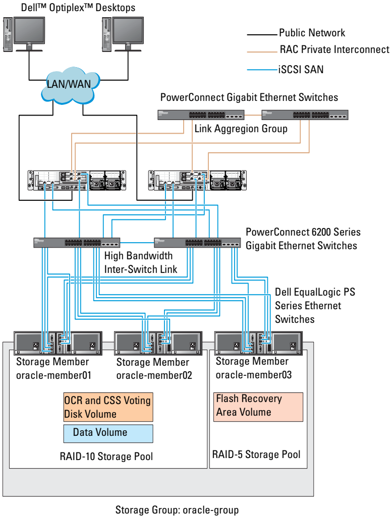
Figure 6-2. Sample Oracle® RAC Configuration with Three PS5000XV Arrays
