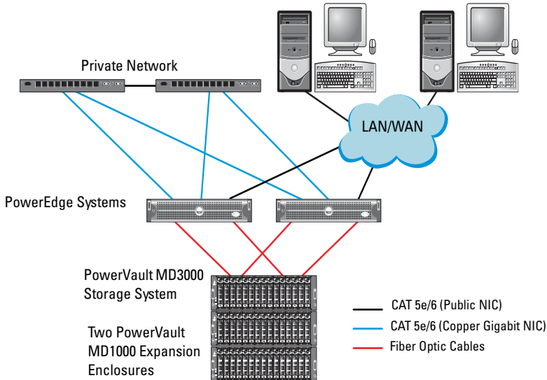
Figure 4-1. Cabling the Serial-Attached SCSI (SAS) Cluster and the Dell PowerVault MD3000 Storage Enclosure
